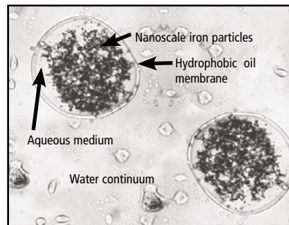
Micrograph of nano-iron emulsion.
